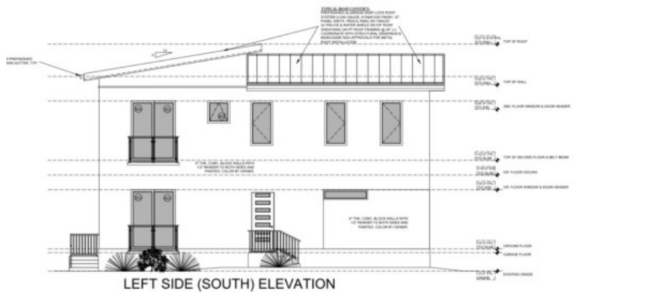
LEFT SIDE (SOUTH) ELEVATION
